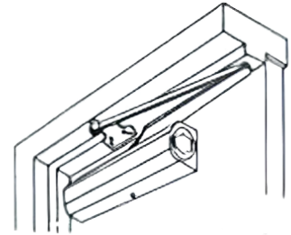
Parallel Mount
