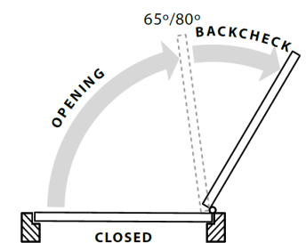
Backcheck
