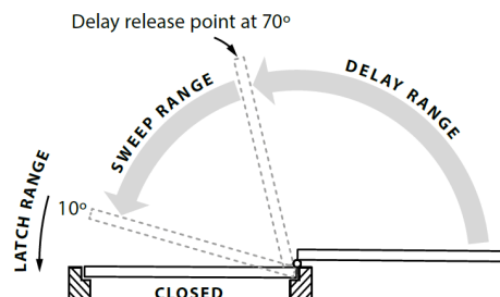
Delayed Action
